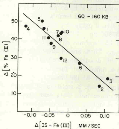
FIGURE 9. Change of ferric isomer shift vs change of conversion [Fe(III) \rightarrow Fe(II)]. Twelve acetylacetonate derivatives.
